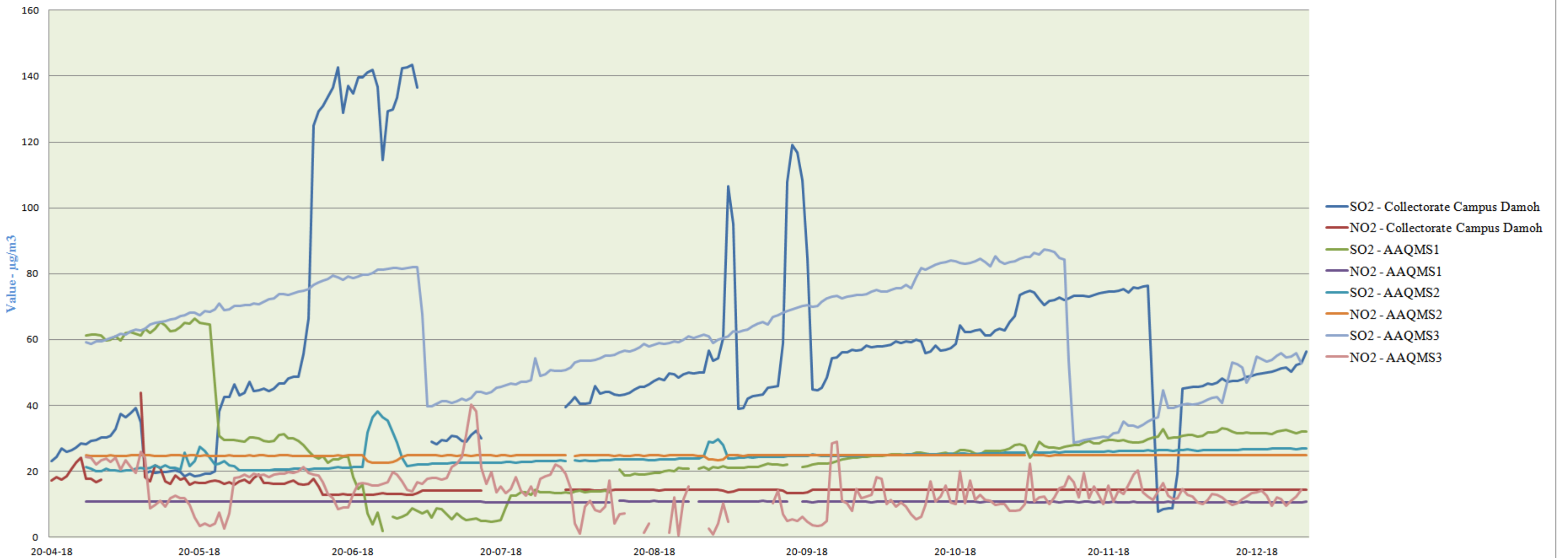
Annual Ambient Trend of Gaseous from M/s Heidelberg Cement India Ltd (Diamond Cements,Clinker Division ) - Narsingarh
