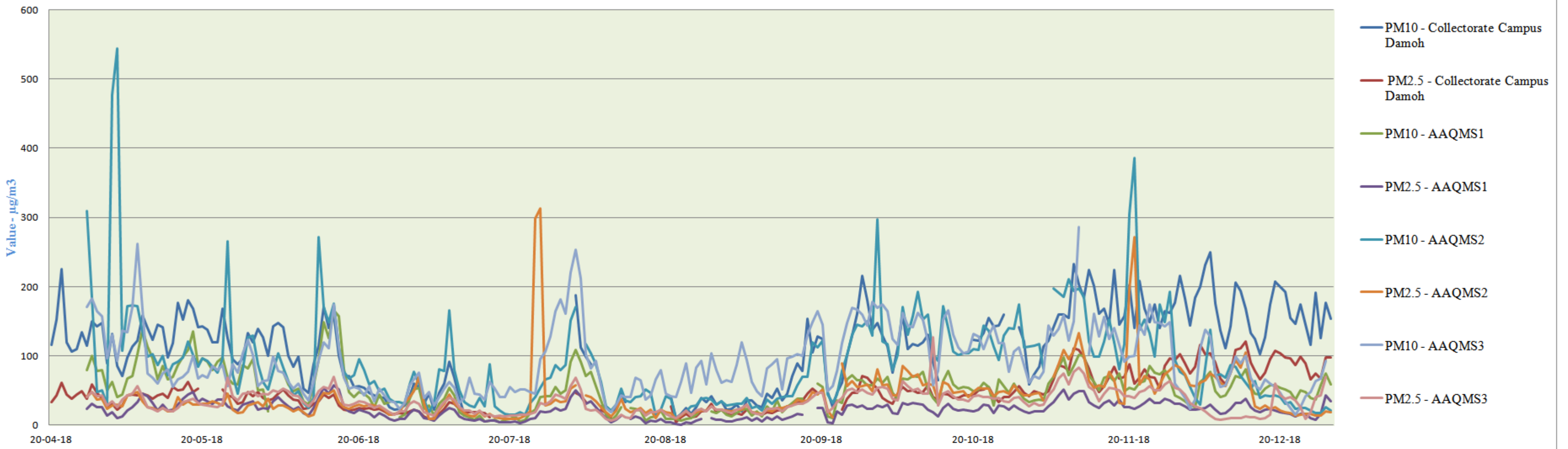
Annual Ambient Trend of PM from M/s Heidelberg Cement India Ltd (Diamond Cements,Clinker Division ) - Narsingarh
